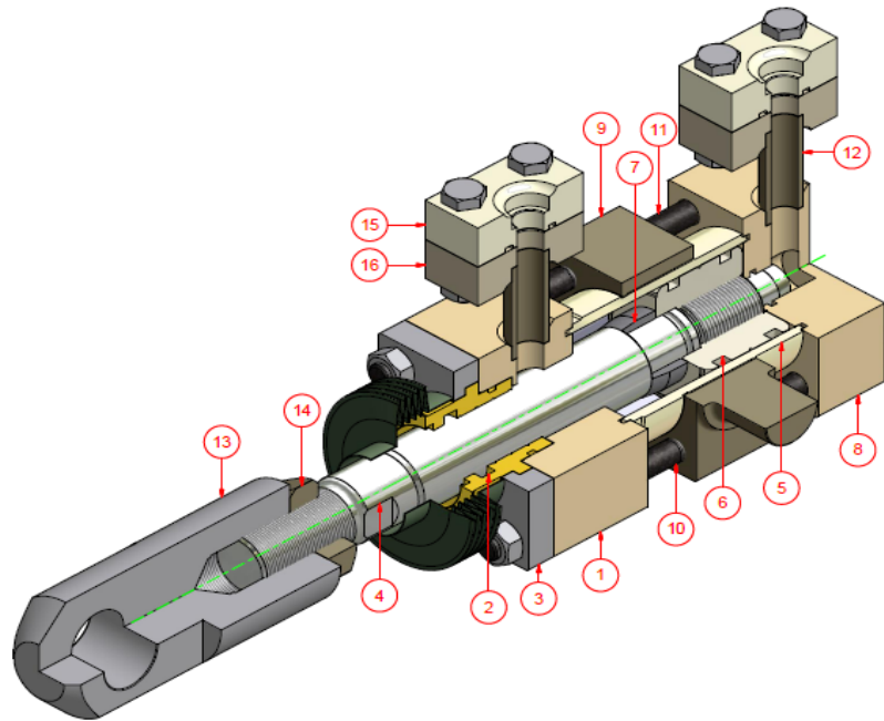
Part List SC-063/036-50-M055
